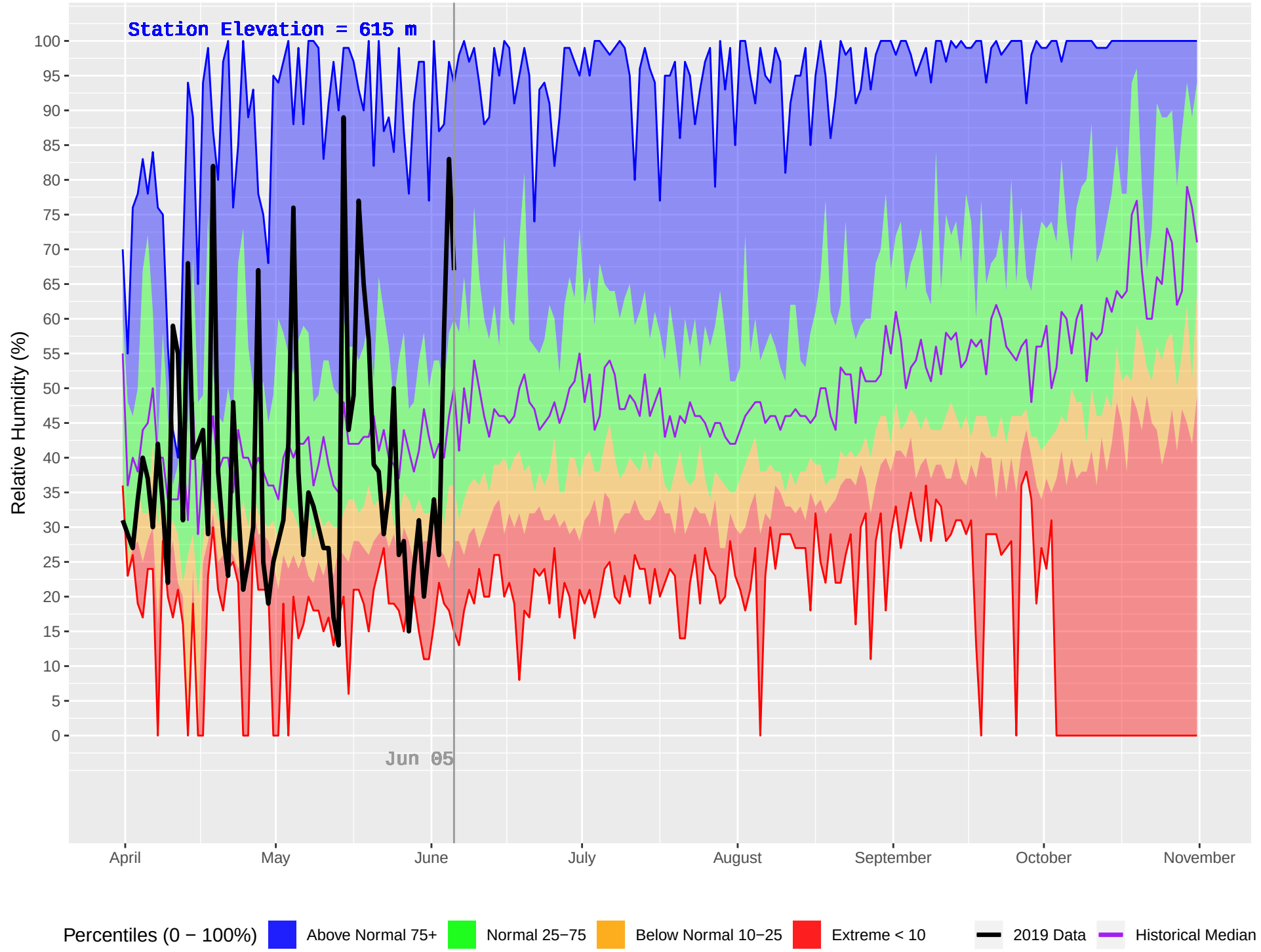
HIXON (187) : Historical (1976–2018) and Current (2019) Daily Relative Humidity
