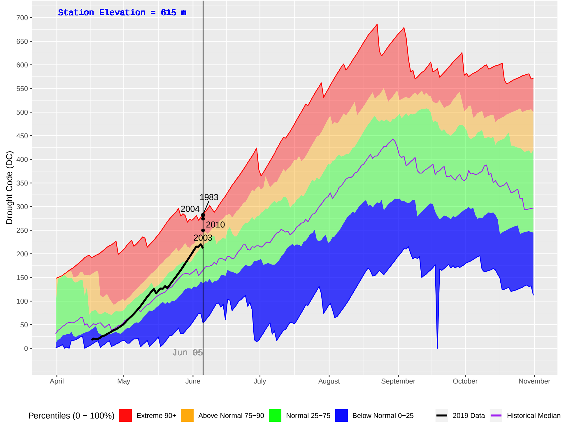
HIXON (187) : Historical (1976–2018) and Current (2019) Daily Drought Code (DC)
