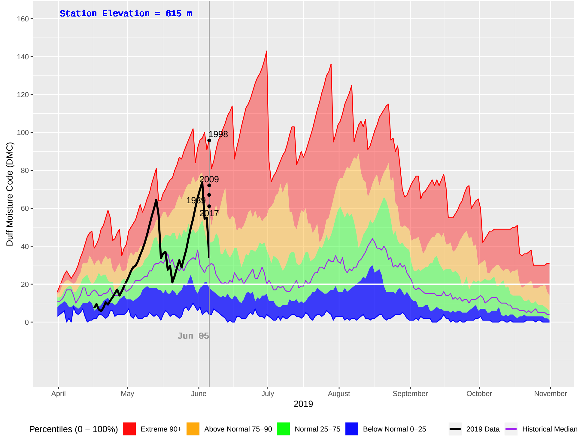
HIXON (187) : Historical (1976–2018), Current (2019) Daily Duff Moisture Code (DMC)
