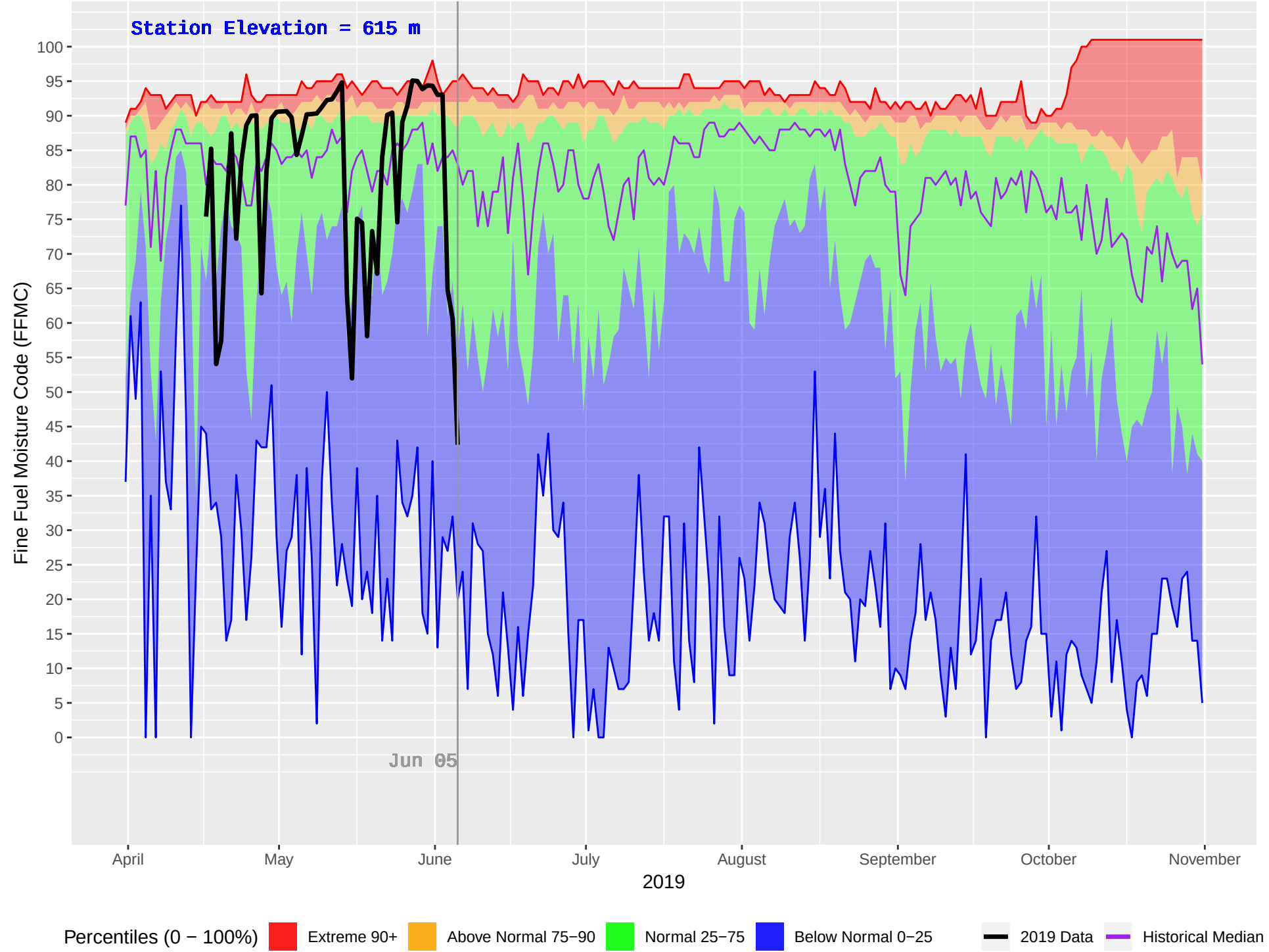
HIXON (187) : Historical (1976–2018) and Current (2019) Daily Fine Fuel Moisture Code (FFMC)
