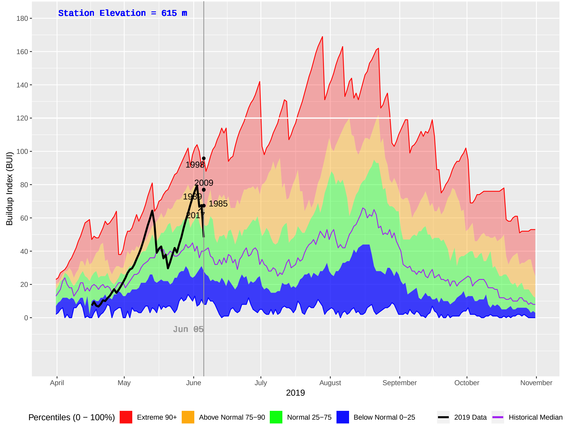
HIXON (187) : Historical (1976–2018), Current (2019) Daily Buildup Index (BUI)
