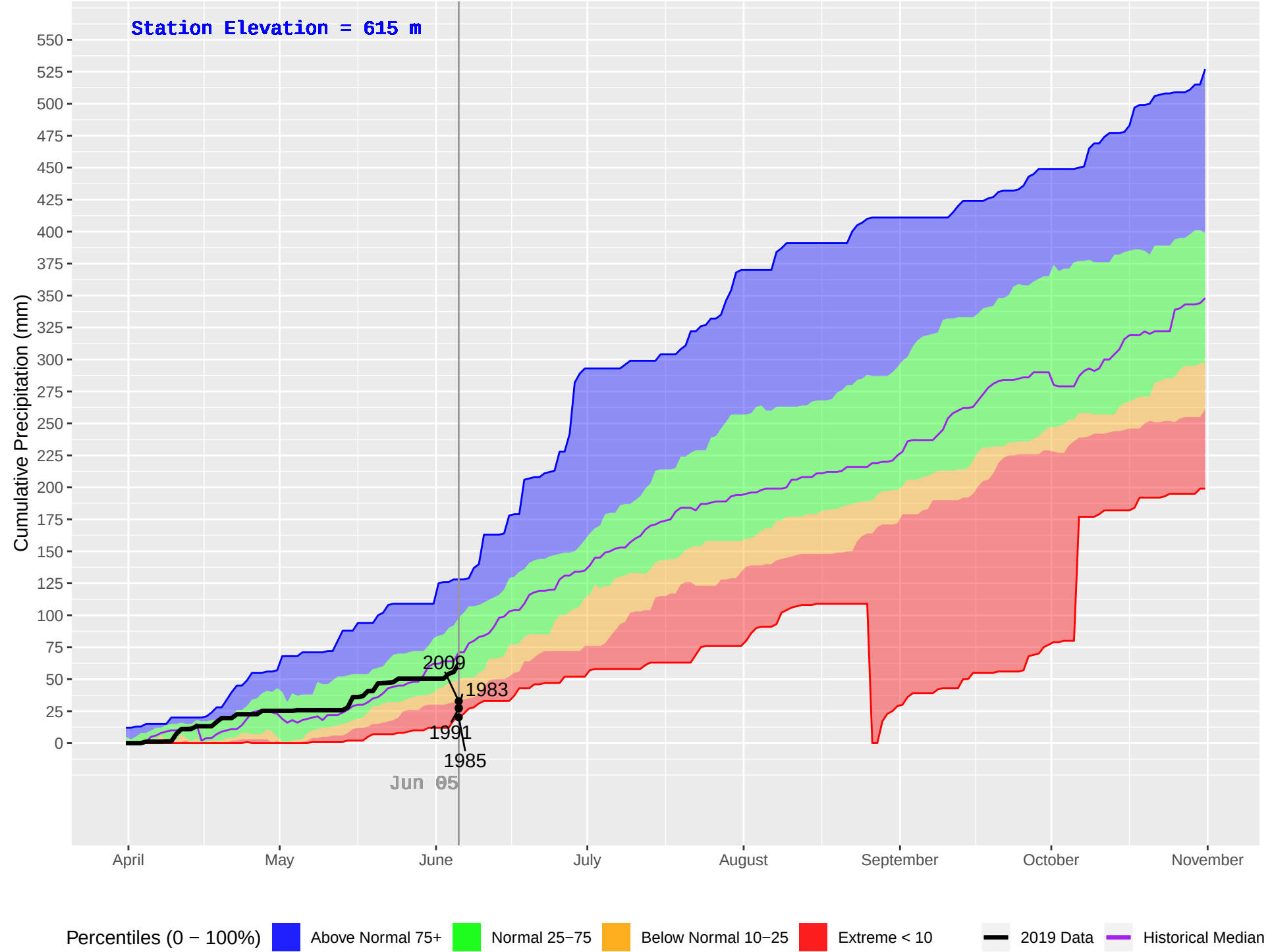
HIXON (187) : Historical (1976–2018), Current (2019) Daily Cumulative Precipitation
